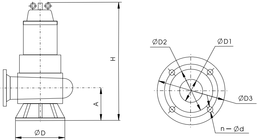
Flange Size
